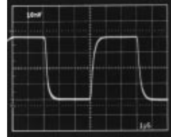
Figure 20. Unity Gain Follower Small Signal Pulse Response
