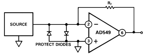
Figure 39. Input Voltage Clamp with Diodes
